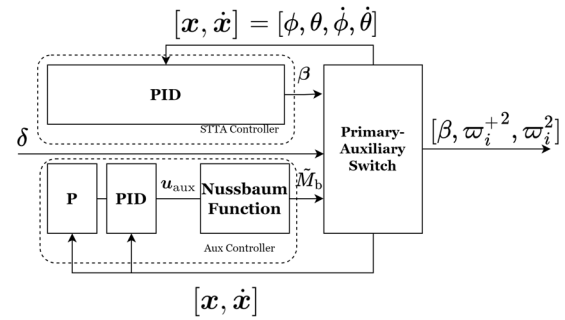
Fig. 4. Detailed scheme diagram of Aqua Slide.
