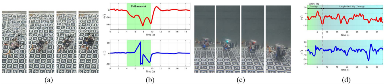
Fig. 12. Comparative physical experiments. (a) Snapshot of the fail moment in the physical experiment without the Nussbaum function. (b) Attitude response during the experiment without Nussbaum function. (c) Snapshot of the moment the vehicle started rolling in the physical experiment without the auxiliary controller. (d) Attitude response during the experiment without the auxiliary controller.
