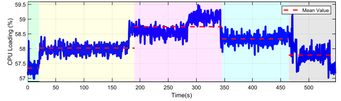
Fig. 8. CPU Loading in the simulation cycle. Sharing the same legends as the Fig. 7.
